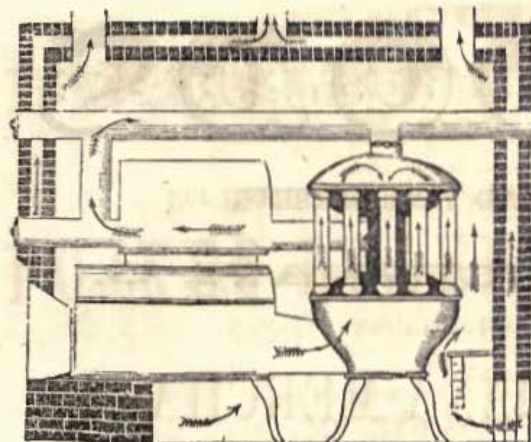
WOOD FURNACE.
