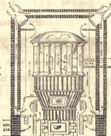
COAL FURNACE.
